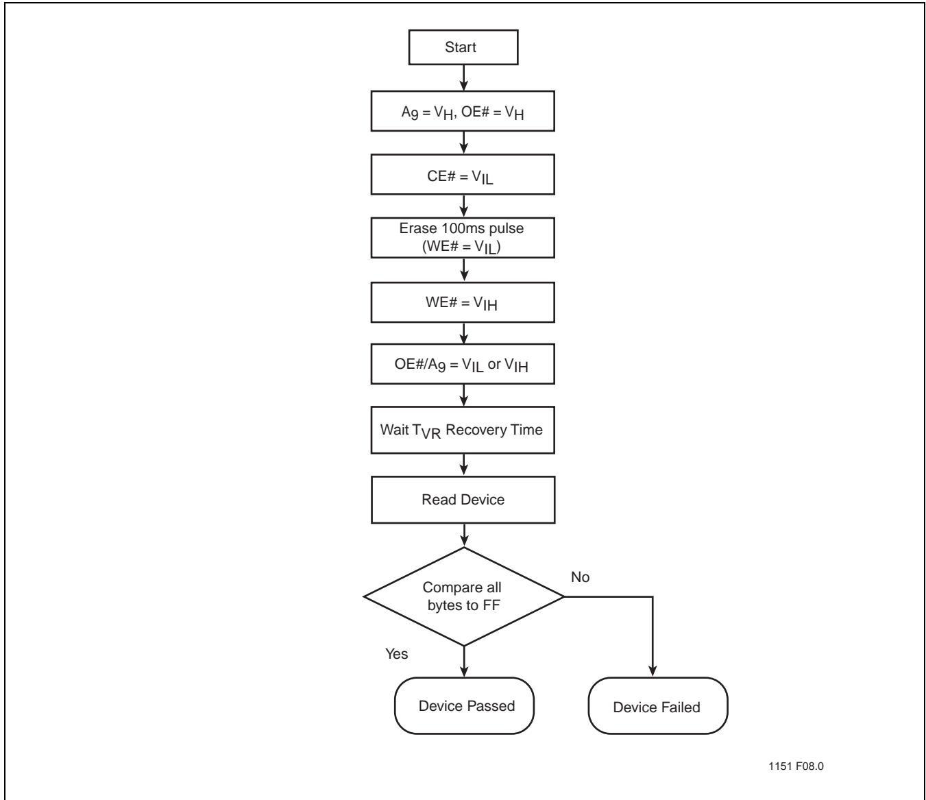
FIGURE 9: CHIP-ERASE ALGORITHM
